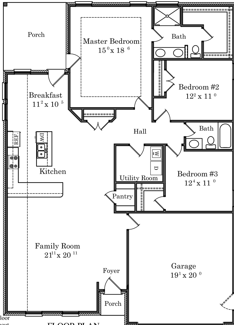
FLOOR PLAN
