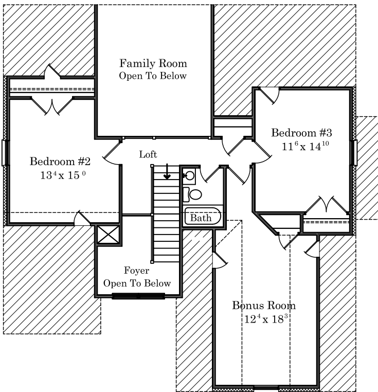
2ND. FLOOR
