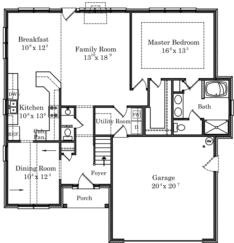
1ST. FLOOR
