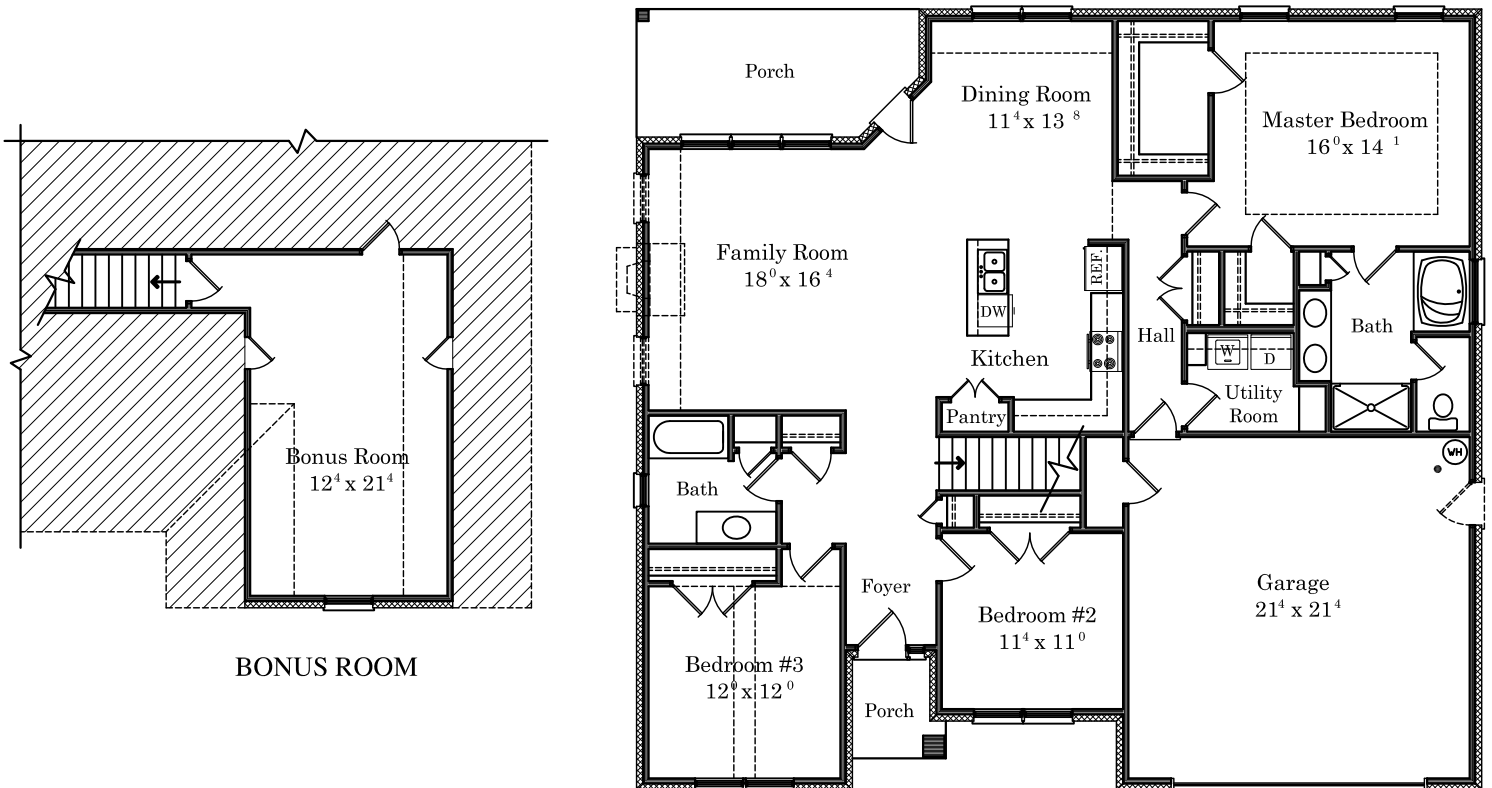
FLOOR PLAN
