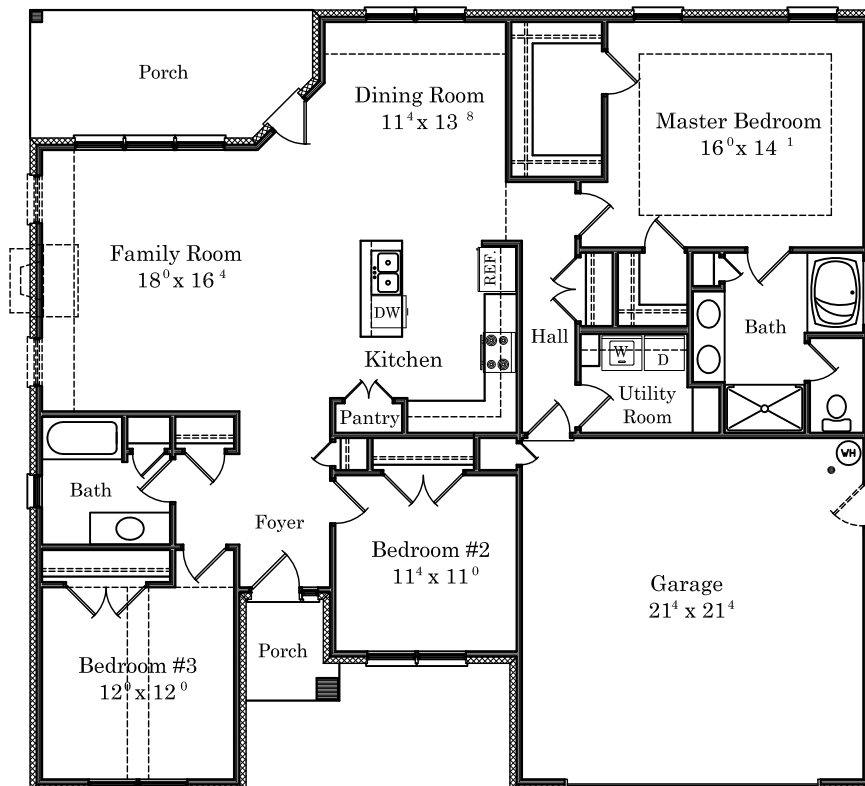
FLOOR PLAN
