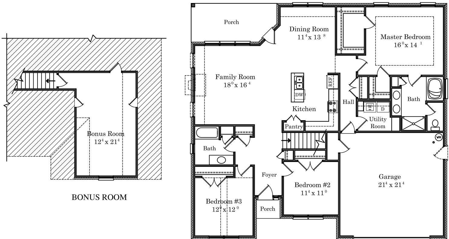
FLOOR PLAN
